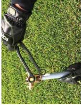
Tightening 9/16", 5/8" & 3/4" fuse nuts
